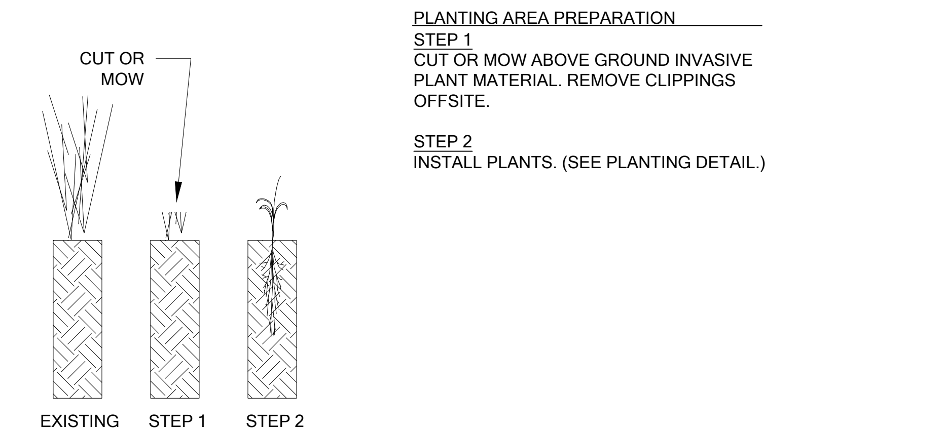
B WETLAND MITIGATION AREA SITE PREPARATION SEE SHEET W1 Scale: NTS
